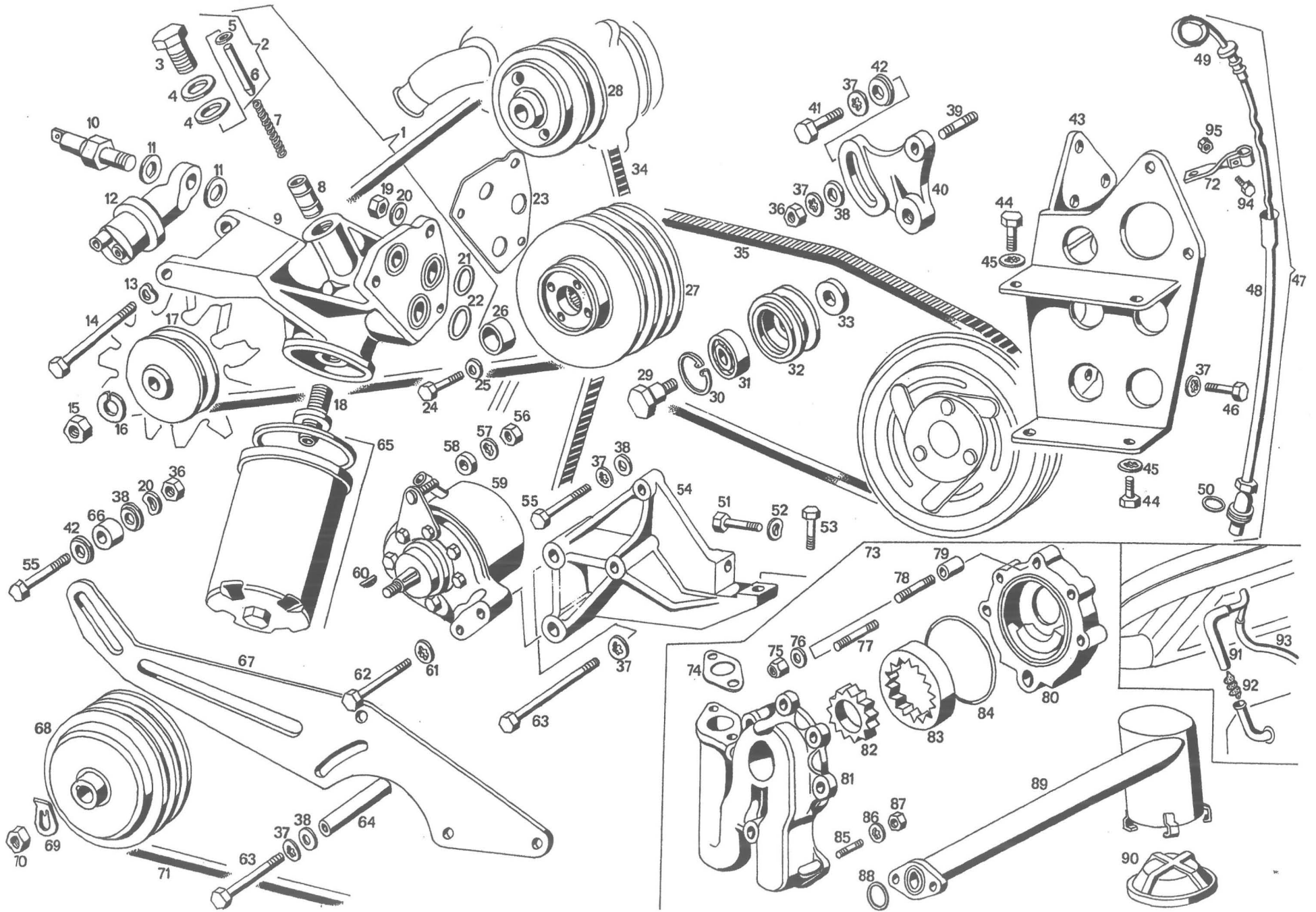
lavola 5 - Pompa olio filtro Table 5 - Oil pump and filter
