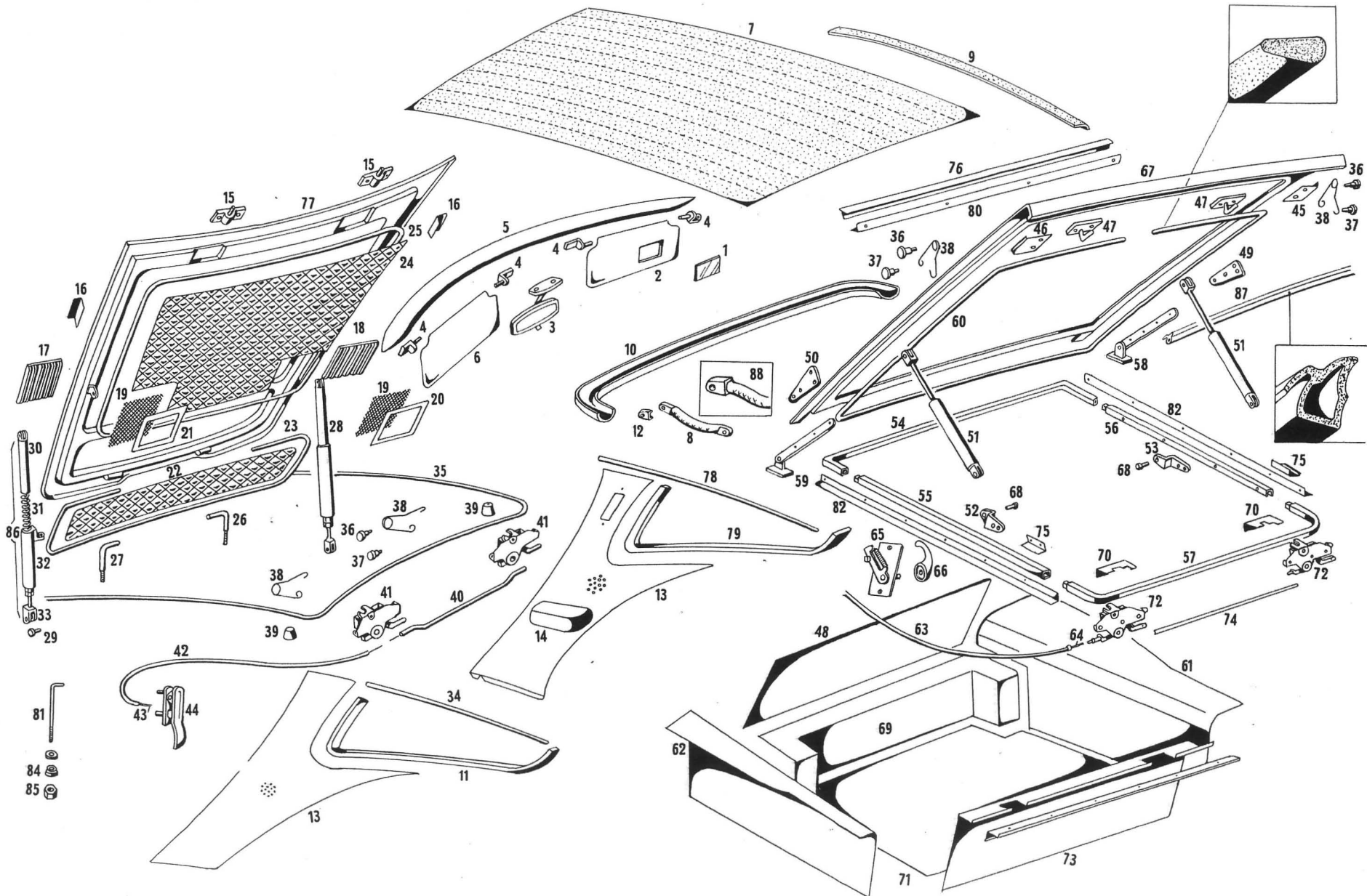
Tavola 41 - Vano motore e baule Table 41 - Engine and Trunk compartment
